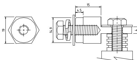
Type H Terminal
